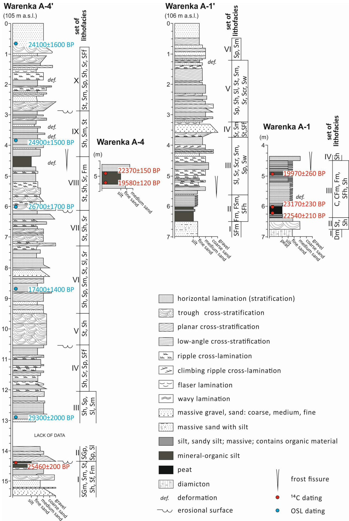
Fig. 3. Lithofacies of sections A-4' and A-1' (modified from Gładys, 2020).
